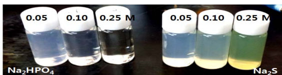
Fig. 3 Photo of precipitating ZnO nanoparticles using Na 2 S and Na 2 HPO 4 with different concentration
