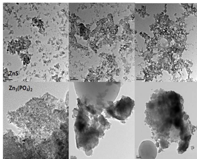
Fig. 5 TEM analysis of precipitated ZnS and Zn 3 (PO 4 ) 2
