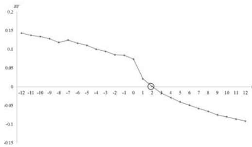
Fig. 1. Bias of Balinski and Young BY(\theta) formulas (3)
