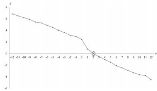
Fig. 3. Bias of B bias measurement B(\theta) formulas (5)
