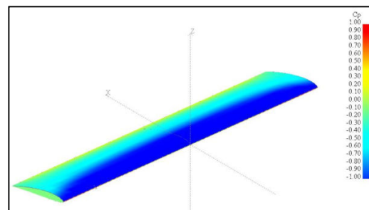
(b) Contours of coefficient of pressure
