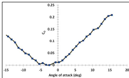
Fig. 5 Variation in C_D with respect to \alpha
