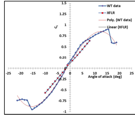
Fig. 6 Variation in C_L with respect to \alpha
