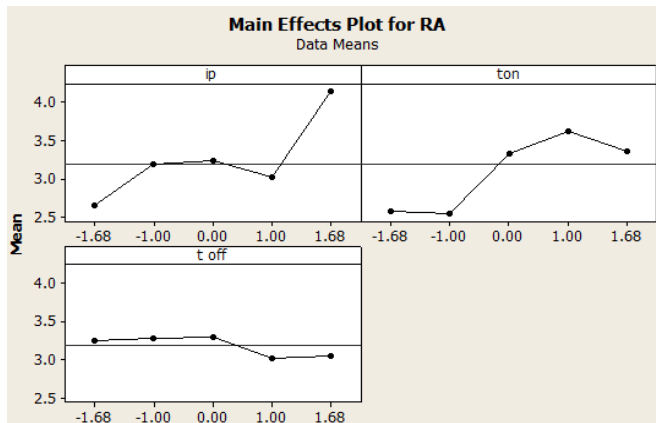
Fig. 5 Main Effect Plots for Surface Finish
