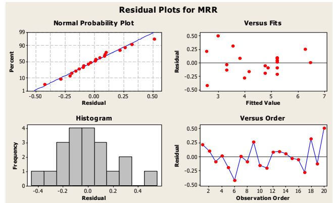
Fig. 2 Residual Plots for Metal Removal Rate
