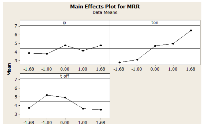
Fig. 4 Main Effect Plots for MRR
