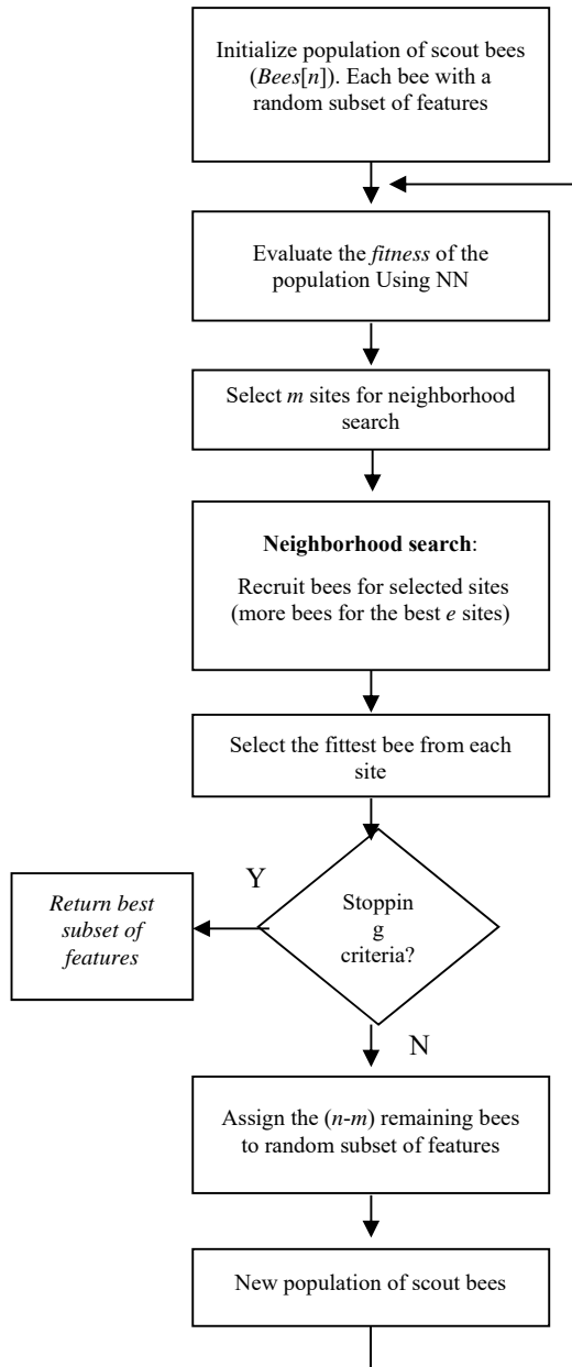
Fig. 3 The general principle of the proposed FS model
