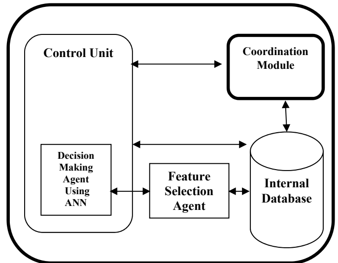
Fig. 2 Internal Architecture of the Proposed Holon
