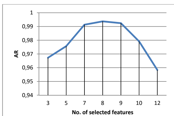
Fig. 5 No. of feature with corresponding AR
