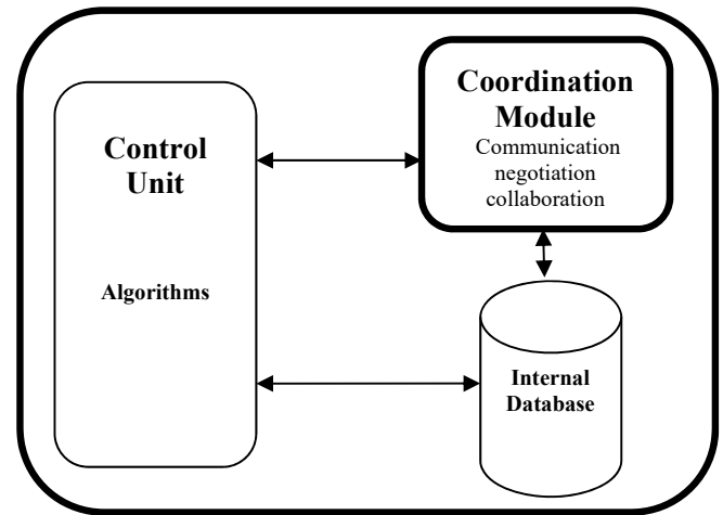
Fig. 1 Internal Architecture of the Basic Holon
