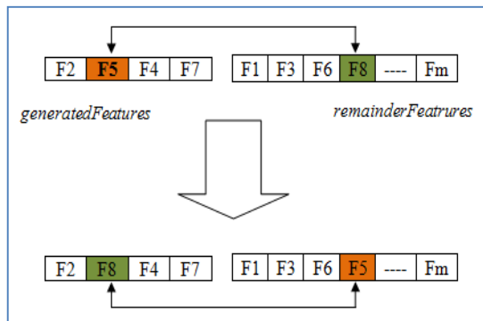
Fig. 4 A simple random exchange operator between generatedFeatures and remainderFeatures
