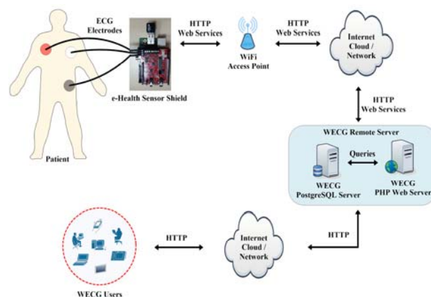
Fig. 2 The block diagram of the WECG measuring and recording system
