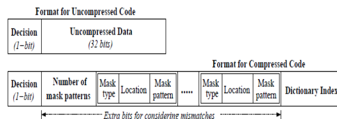
Fig. 2 Encoding format for bit masking compression technique
