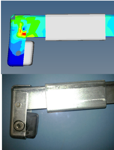
Fig. 6 Corresponded plastic deformation of bracket
