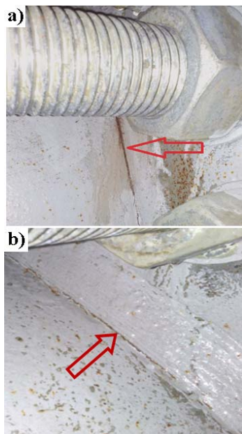
Fig. 3 Crack formation in pipe-plate welding zones
