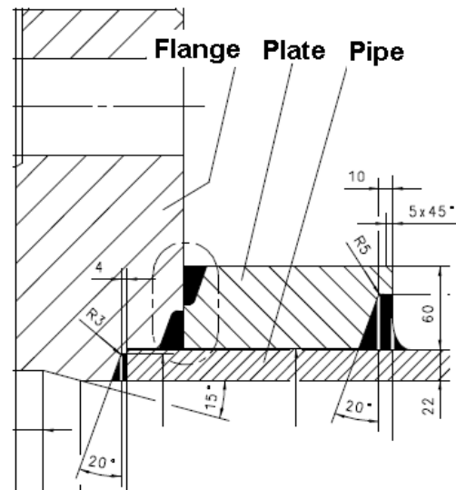
Fig. 5 Technical drawing of the pipe-plate-flange system
