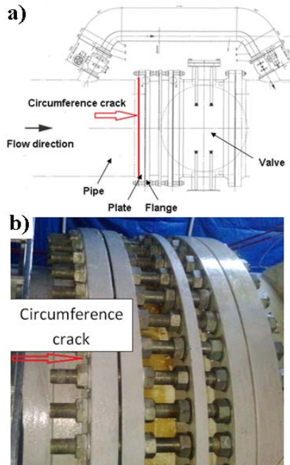
Fig. 2 General view of the flange-plate-pipe system and circumference crack
