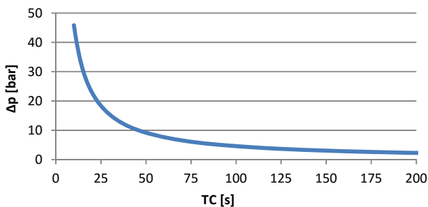
Fig. 6 Relation between pressure rise due to water hammer ( \Delta p ) and time to close the main valve ( T_C )
