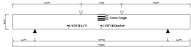
Fig. 3 Detail of gages and LVDT when loading
