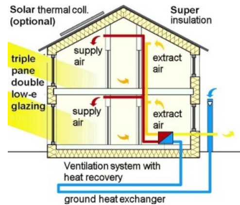
Fig. 4 Passive house
