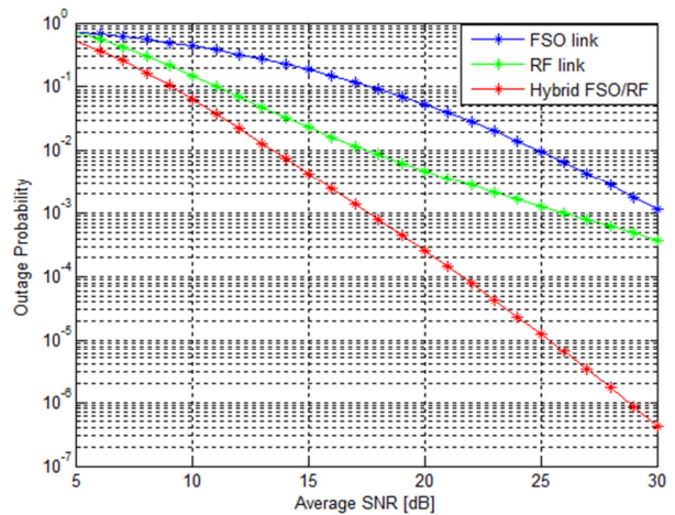
Fig. 9 Outage probability over atmospheric turbulence \beta^2=0.8
