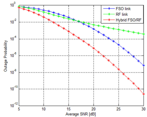
Fig. 8 Outage probability over atmospheric turbulence \beta^2=0.5
