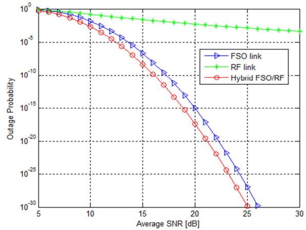
Fig. 7 Outage probability over atmospheric turbulence \beta^2=0.3
