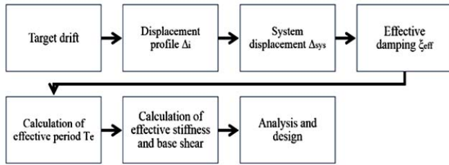
Fig. 4 Design methodology of DDBD
