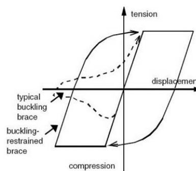
Fig. 3 Force-displacement behavior between BRB and traditional braces
