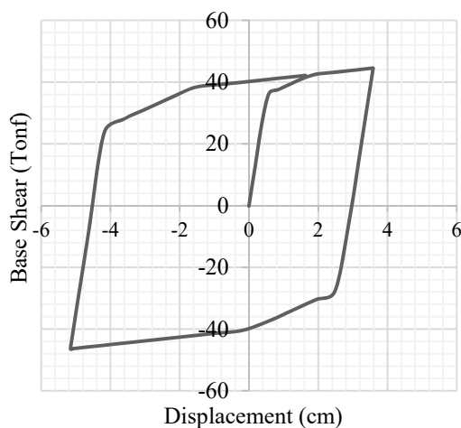
Fig. 18 Single BRB hysteresis curve
