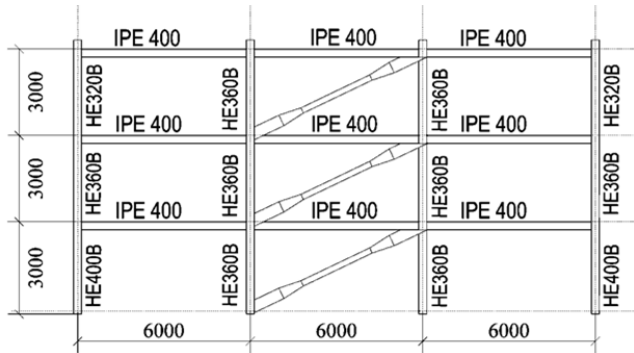
Fig. 8 Dual moment steel frame with BRB
