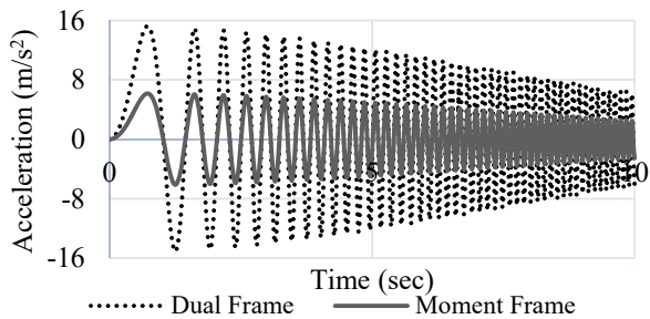
Fig. 12 Sweep wave loading
