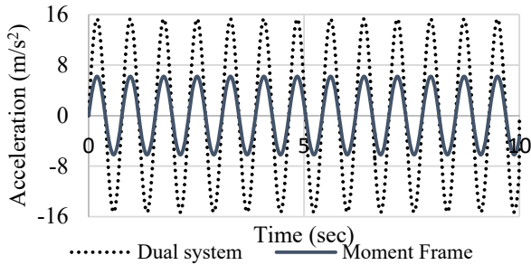
Fig. 11 Harmonic loading
