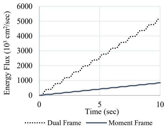
Fig. 13 Energy Flux
