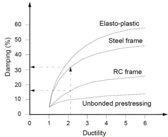
Fig. 6 EVD vs ductility
