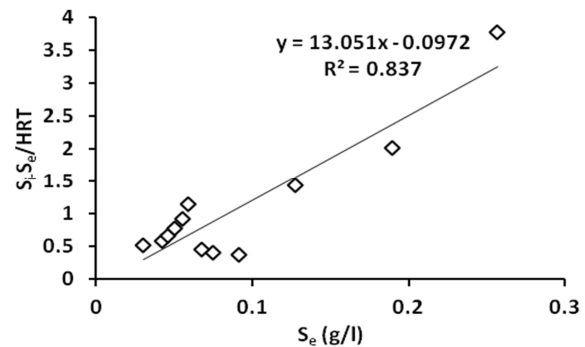
Fig. 5 First order kinetic model plot
