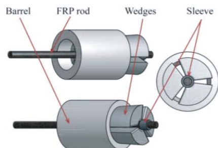
Fig. 1 Wedge anchorage system components
