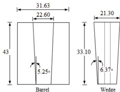
Fig. 2 Wedge dimensions in millimeters
