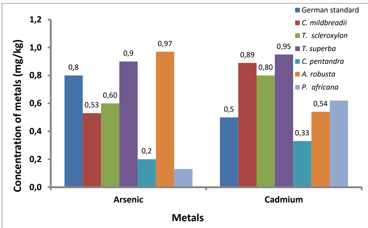
Fig. 2 Concentration of Arsenic and Cadmium in sawdust of six tropical hardwood species
