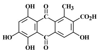
Fig. 2 Representative molecular structure of natural dyes, anthraquinone
