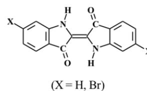
Fig. 1 Representative molecular structure of natural dyes, indigoid
