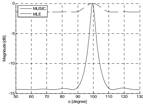
Fig. 3 MLE and MUSIC Spectrum
