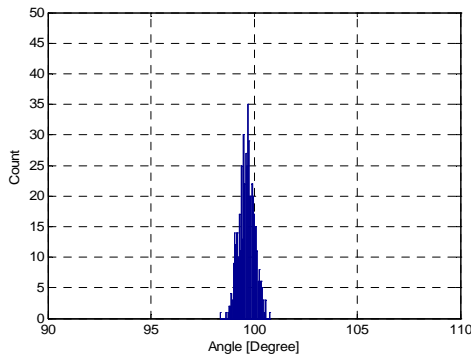
Fig. 4 Histogram Based on 500 Independent Trials
