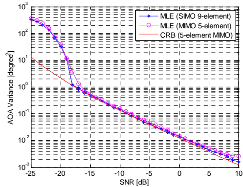
Fig. 5 AOA Estimation Variance
