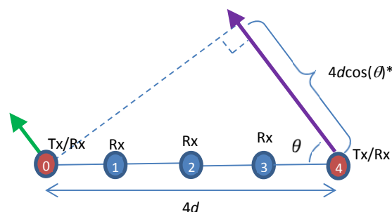
Fig. 1 MIMO Transmitter/Receiver
