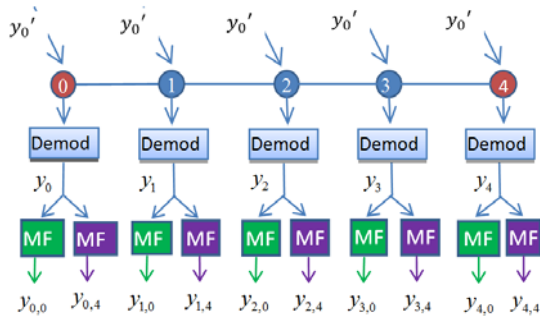
Fig. 2 MIMO Receiver
