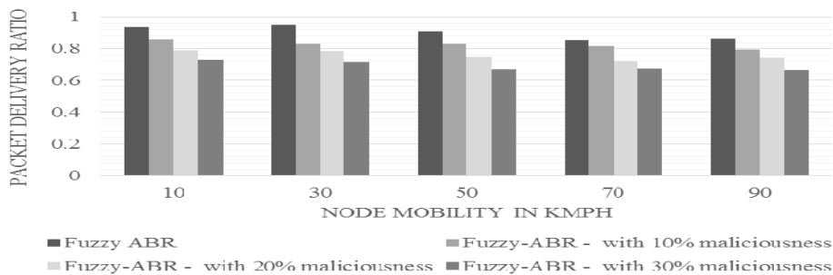
Fig. 8 Packet Delivery Ratio for Fuzzy ABR
