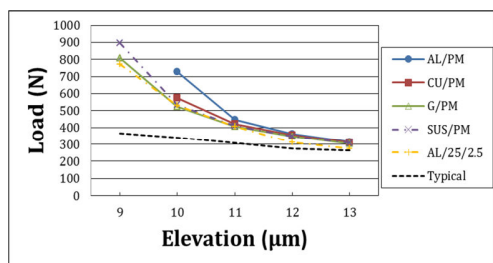
Fig. 6 Load vs. elevation for different structure and material combinations. AL/PM represents polymer body covered by aluminum alloy 6061, etc.; AL/25/2.5 denotes 2.5 mm-thick AL disk supported at radius 25 mm
