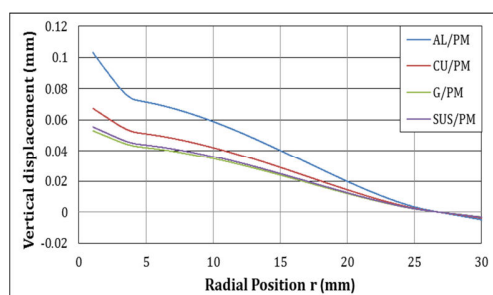
Fig. 8 Vertical displacement of the disk bearing surface, measured from the center to the brim of the disk at elevation 10 µm
