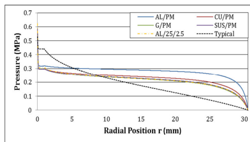
Fig. 9 Air pressure distribution along the bearing surface, measured from the center to the brim of the disk at elevation 10 µm
