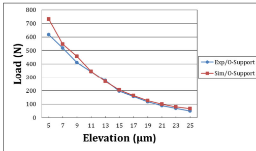
Fig. 4 Comparison between simulation (red) and experimental (blue) results
