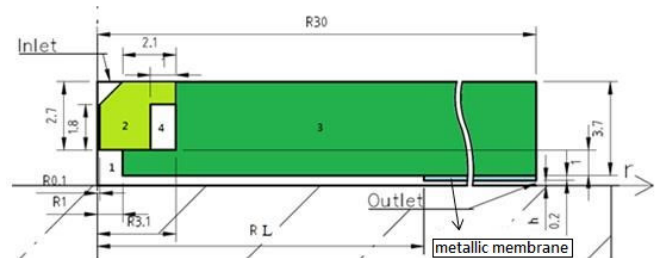
Fig. 1 Polymer body with metal membrane at bottom [5]; the bearing is supported on the tops of components 2 and 3
