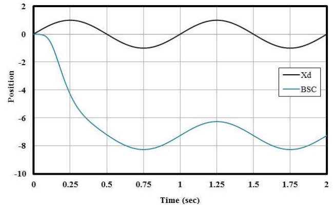
Fig. 6 Simulation of piston position tracking for standard back-stepping controller with disturbances
