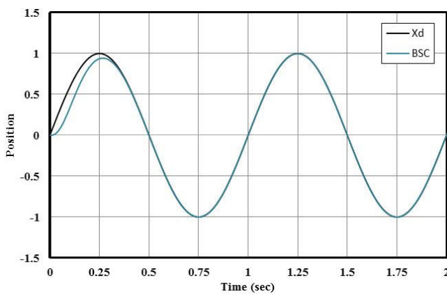
Fig. 4 Simulation of piston position tracking for standard back-stepping controller in the absence of disturbances and uncertainties
