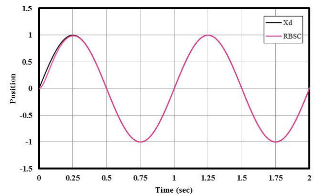
Fig. 7 Simulation of piston position tracking for robust back-stepping controller with disturbances
