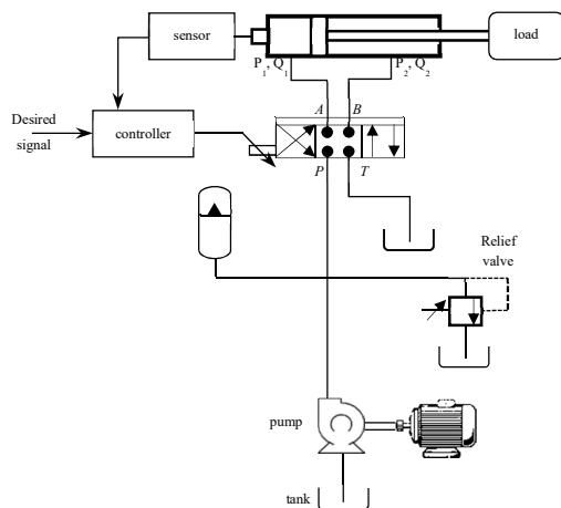
Fig. 1 Typical electro-hydraulic servo system
