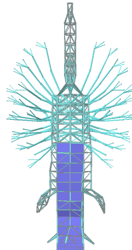
Fig. 12 FEM model of inner primary structure
