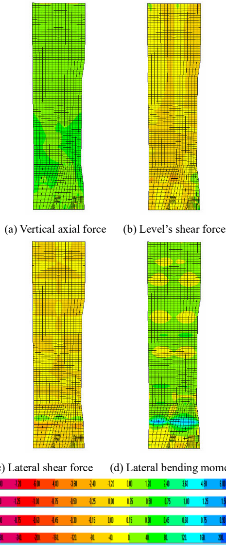
Fig. 21 Internal force diagram of \circ ,Aaxis wall in +Y direction wind load case
