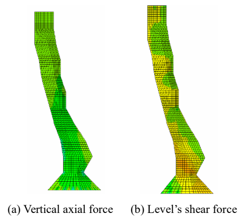
Fig. 19 Internal force diagram of \circ, A axis wall in +X direction wind load case
