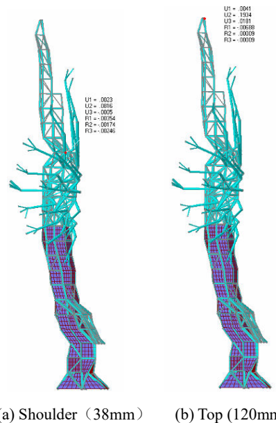
Fig. 17 The max displacement in load cases 3
