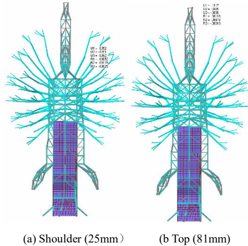
Fig. 15 The max displacement in load cases 1
