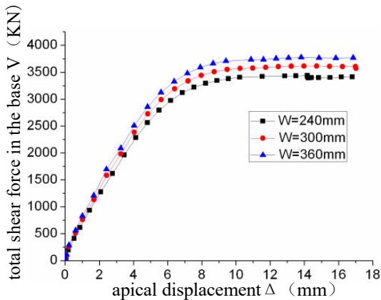
Fig. 7 The W influences to load-displacement curve
