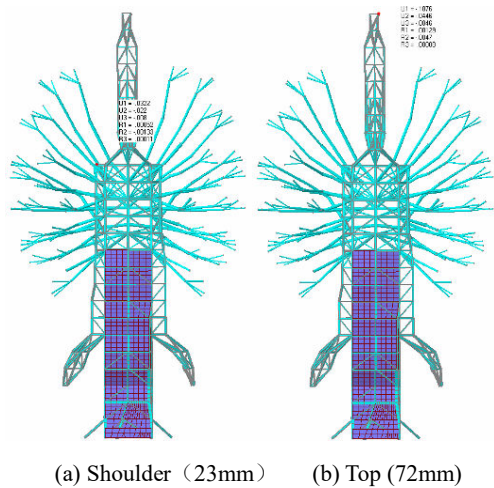
Fig. 16 The max displacement in load cases 2
