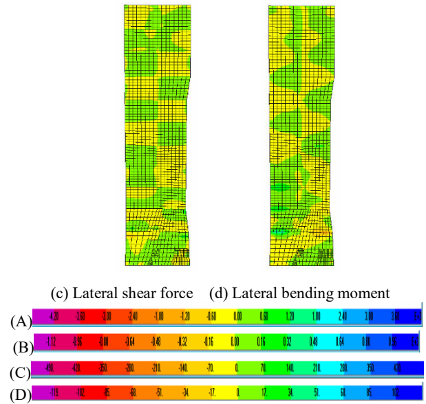
Fig. 19 Internal force diagram of \circ, A axis wall in +X direction wind load case
