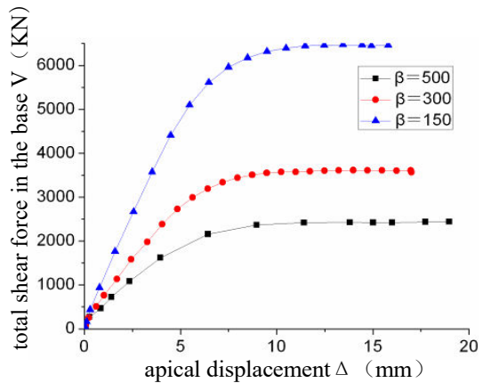
Fig. 5 The \beta influences to load-displacement curve
