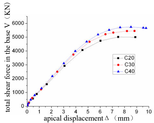
Fig. 9 The influences of strength grade of the concrete to load-displacement curve
