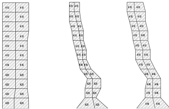
(a) Front wall of 0,A axis (b) Side wall of ④axis (c) Side wall of ③axis Fig. 14 The cross-section distribution of Steel-concrete Composite Shear Wall
