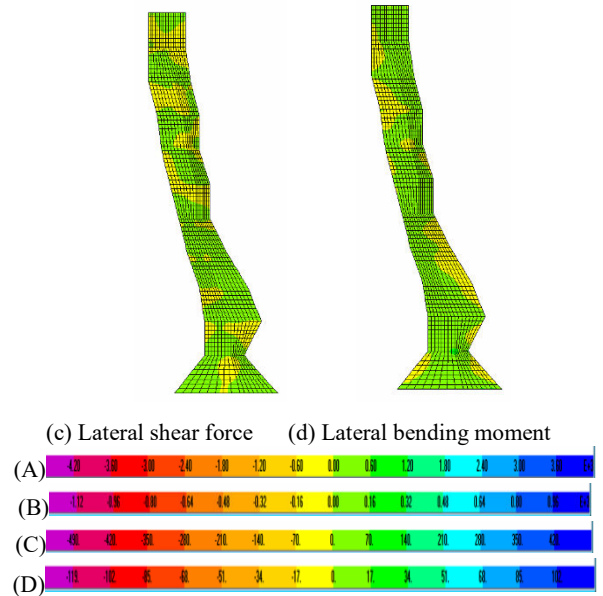
Fig. 20 Internal force diagram of \circ, 2 axis wall in +X direction wind load case
