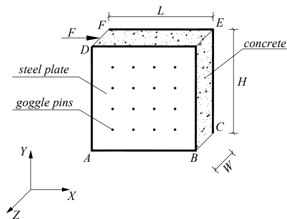
Fig. 1 Application of load and correlative parameters of twin steel plates-concrete composite shear wall
