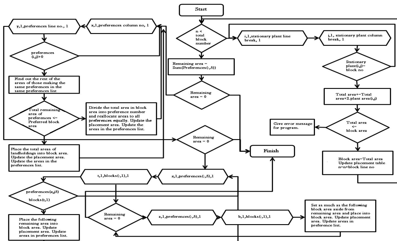
Fig. 4 Flow Chart of Block Reallocation Algorithm
