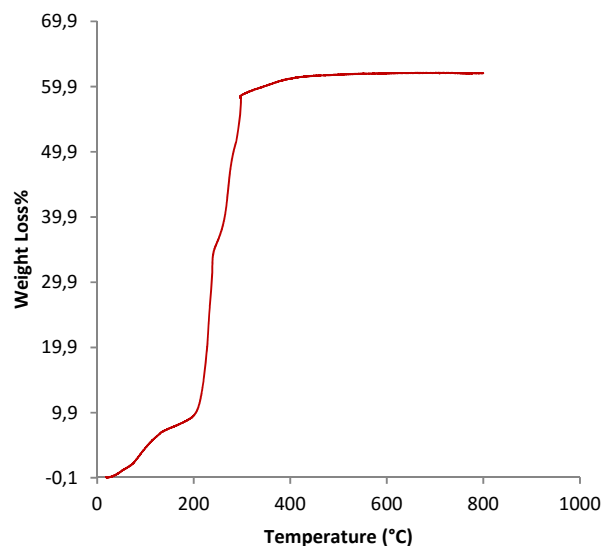
Fig. 1 Thermal Analysis (TGA) of thoria dried gel
