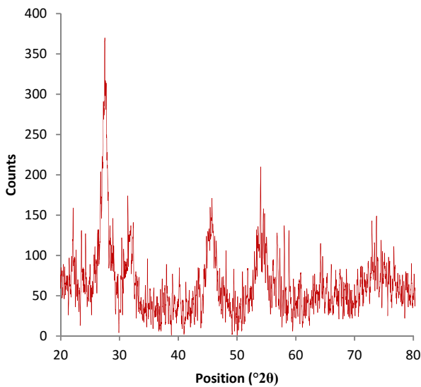
Fig. 4 XRD analysis of prepared thoria powder
