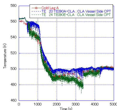
Fig. 4 Cold-Leg Fluid Temperatures in Intact Loop
