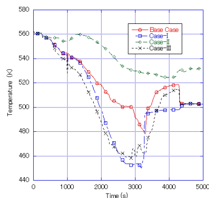
Fig. 8 Cold-Leg Fluid Temperatures in Broken Loop
