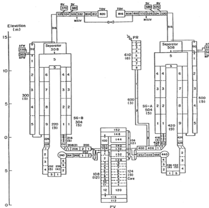
Fig. 2 LSTF Input Model
