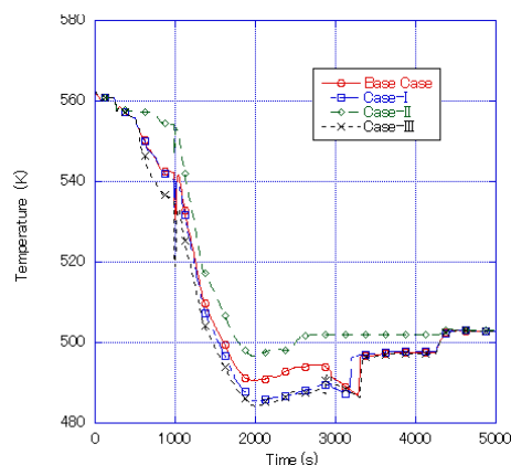
Fig. 7 Cold-Leg Fluid Temperatures in Intact Loop
