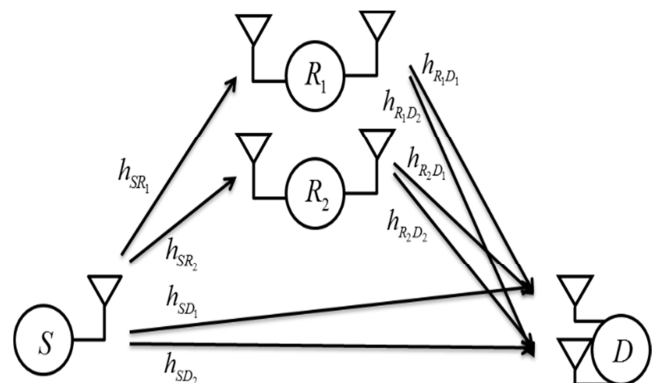
Fig. 1 A cooperative relay system
