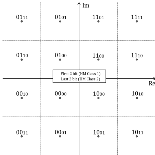
Fig. 2 The constellation for hierarchical modulation
