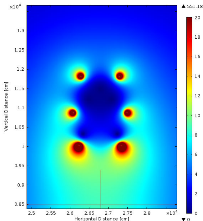
Fig. 2 Electric field distribution in kV/m around Type II pylon
