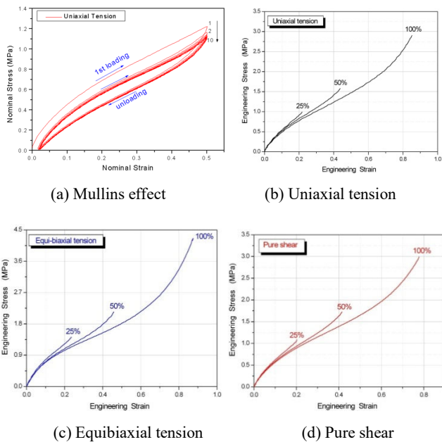
Fig. 3 Stress-strain curve at various strain range
