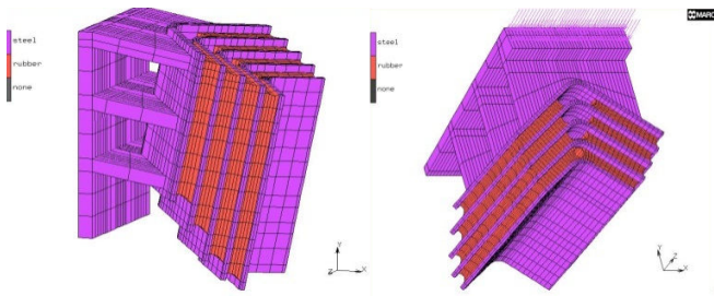
Fig. 4 Finite element model of chevron rubber spring
