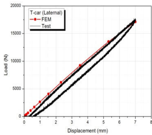
(c) Lateral direction
