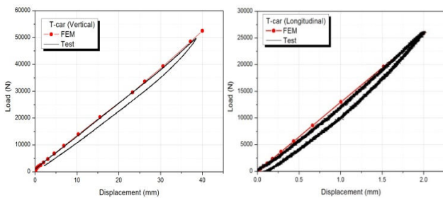
(a) Vertical direction (b) Longitudinal direction
