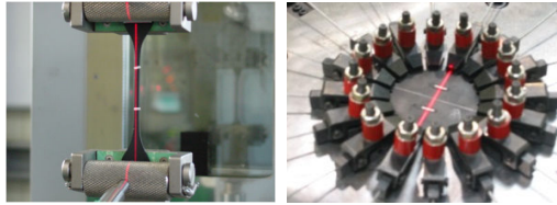
(a) Uniaxial tension test (b) Equibiaxial tension test
