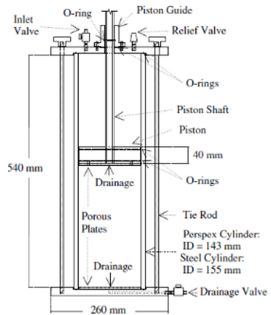
Fig. 2 Sketch of enlarged consolidation cell by [6]
