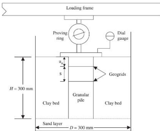
Fig. 1 Experimental setup by [5]
