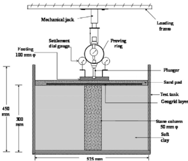
Fig. 4 Schematic diagram of the test setup by [7]
