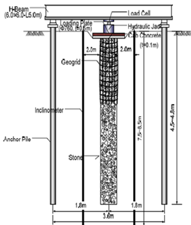
Fig. 7 Load test and measurement equipment
