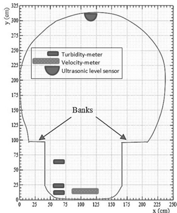
Fig. 1 Sewer Section Details and Measurement Equipment Position
