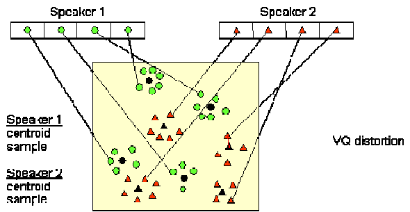
Fig. 10 Conceptual diagram illustrating VQ codebook formations
