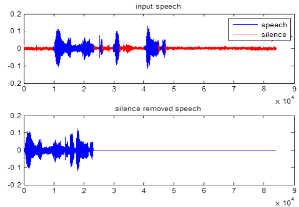
Fig. 4 Silence removal by hybrid algorithm
