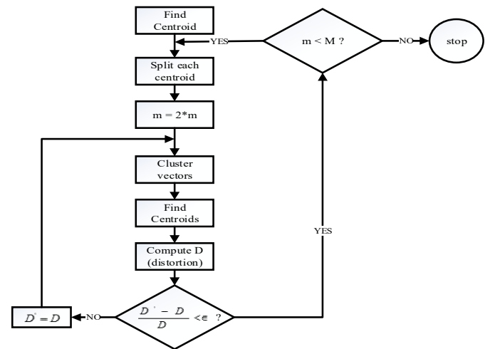
Fig. 11 Flow diagram of the LBG algorithm
