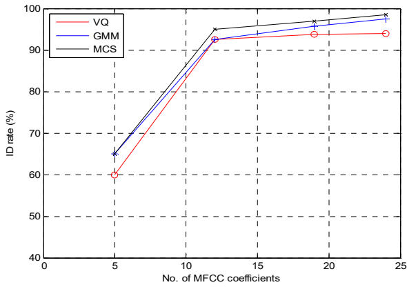
Fig. 17 Identification rate as a function of the number of the MFCC coefficients. Using 29 filter, a codebook size of 128 and 16 Gaussian mixture components
