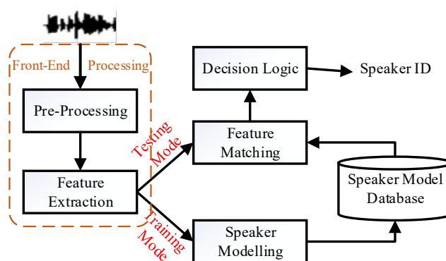
Fig. 1 Basic structure of Speaker Identification (SI)
