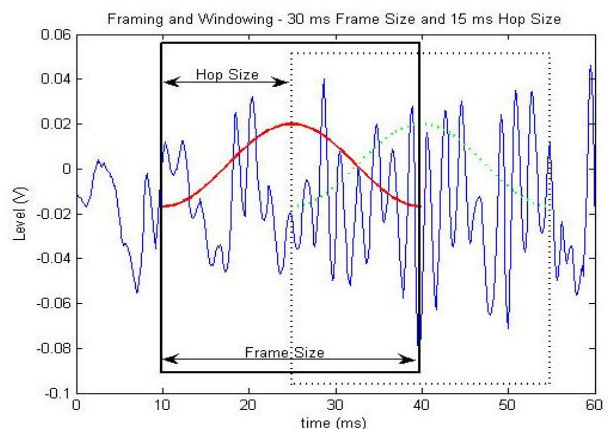
Fig. 5 Speech frame blocking and windowing
