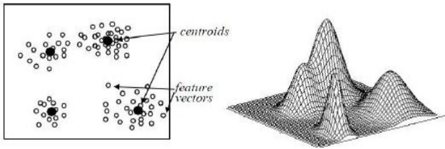
Fig. 12 GMM models showing a feature space and corresponding Gaussian model in 2D
