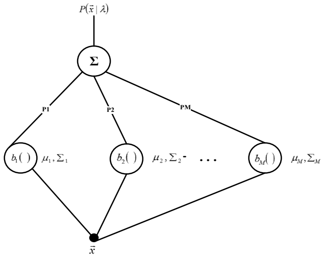
Fig. 13 Description of M-component Gaussian densities
