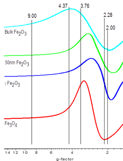
Fig. 7 EPR spectrum of iron oxide standards (10 \mu g transferred in 4mm EPR tube). Standards of both Fe(III)_2O_3 and Fe_3O_4 exhibited a large broad singlet peak with no fine structure which is typical at elevated concentrations
