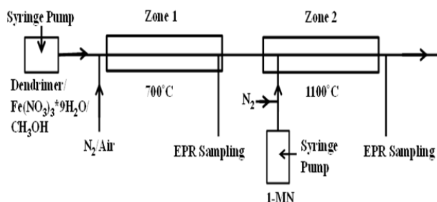
Fig. 1 Schematic of experimental dual zone reactor
