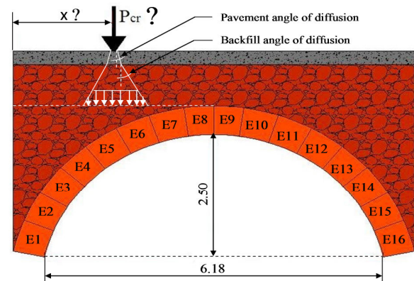
Fig. 2 Loading model
