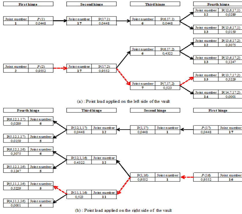
Fig. 7 Probability of hinges appearance ( CV = 20\% )
