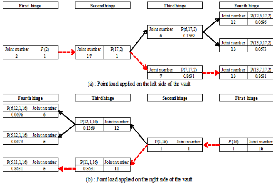
Fig. 5 Probability of hinges appearance ( CV = 5\% )
