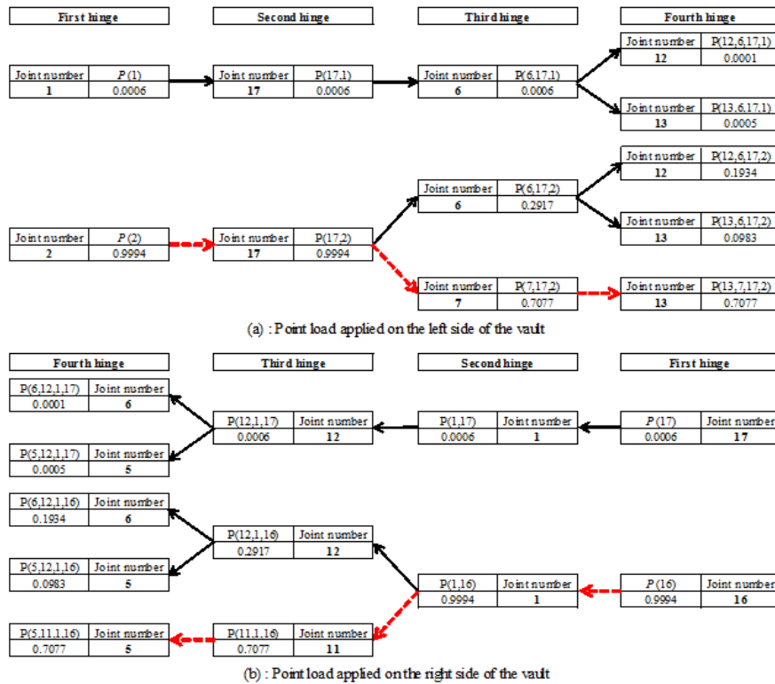
Fig. 6 Probability of hinges appearance ( CV = 10\% )
