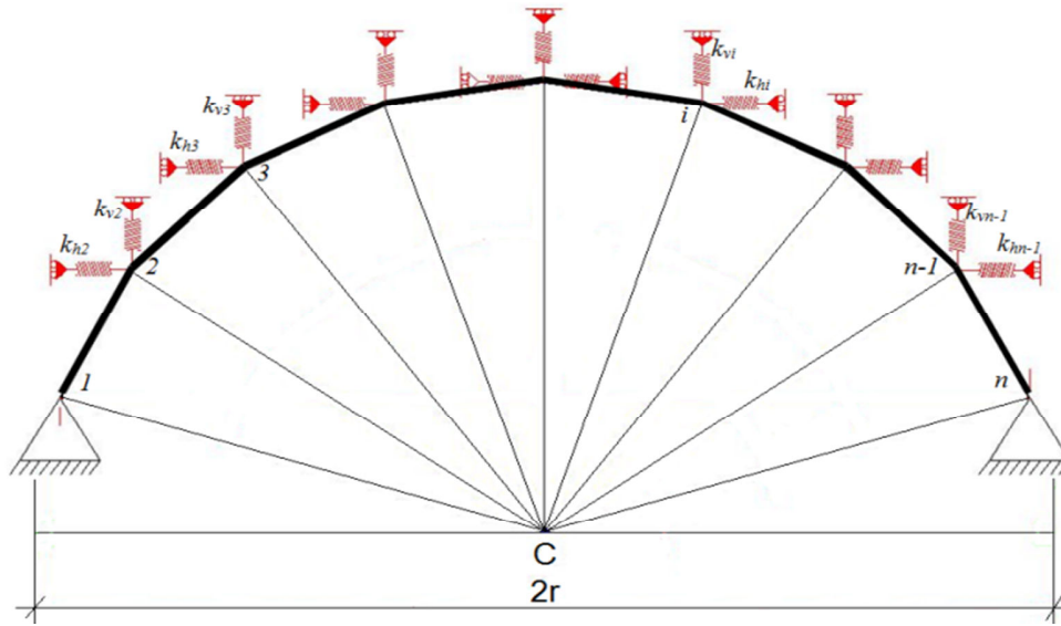
Fig. 1 Modeling of backfill reaction (ArcProg_Z)
