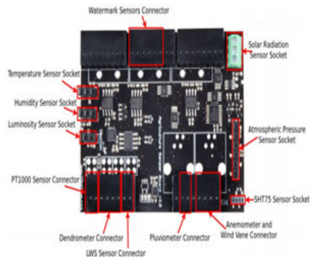
Fig. 2 Waspote Agriculture Sensor Board PRO
