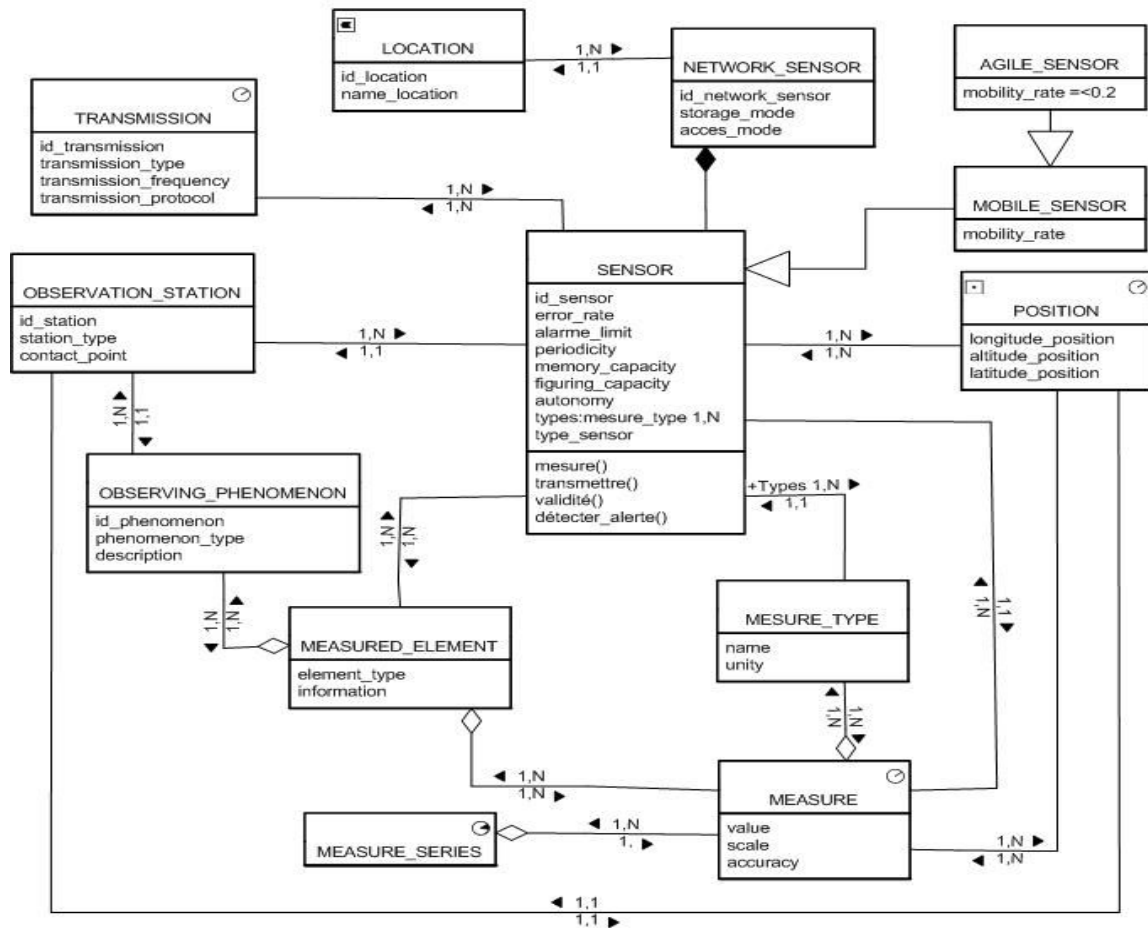
Fig. 3 Real-Time Spatio-Temporal Data Model (adapted from [16])
