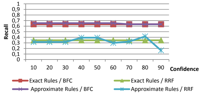
Fig. 11 Variation of recall rates associated to exact and approximate rules after partial mapping using BFC's and RRF's classifiers
