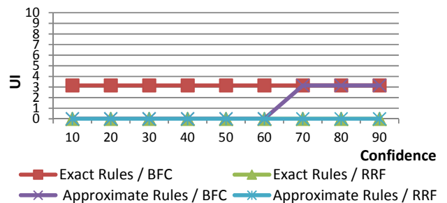
Fig. 14 Variation of UI rates associated to exact and approximate rules after partial mapping using BFC's and RRF's classification rules
