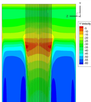
Fig. 11 Y velocity contours of attenuator containing fibers
