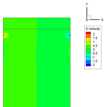
Fig. 6 Attenuator simulation X velocity results
