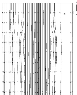
Fig. 10 Air flow vectors of attenuator containing fibers
