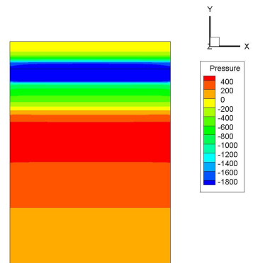
Fig. 7 Attenuator simulation pressure results
