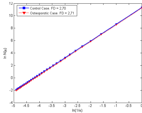
Fig. 6 Fractal dimension calculation, using the box counting method applied to the trabecular images segmentation
