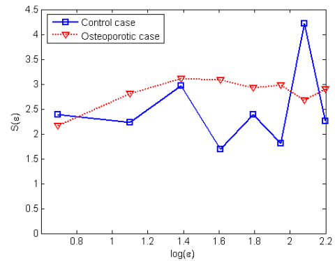
Fig. 8 Fractal signature for the trabecular segmentation
