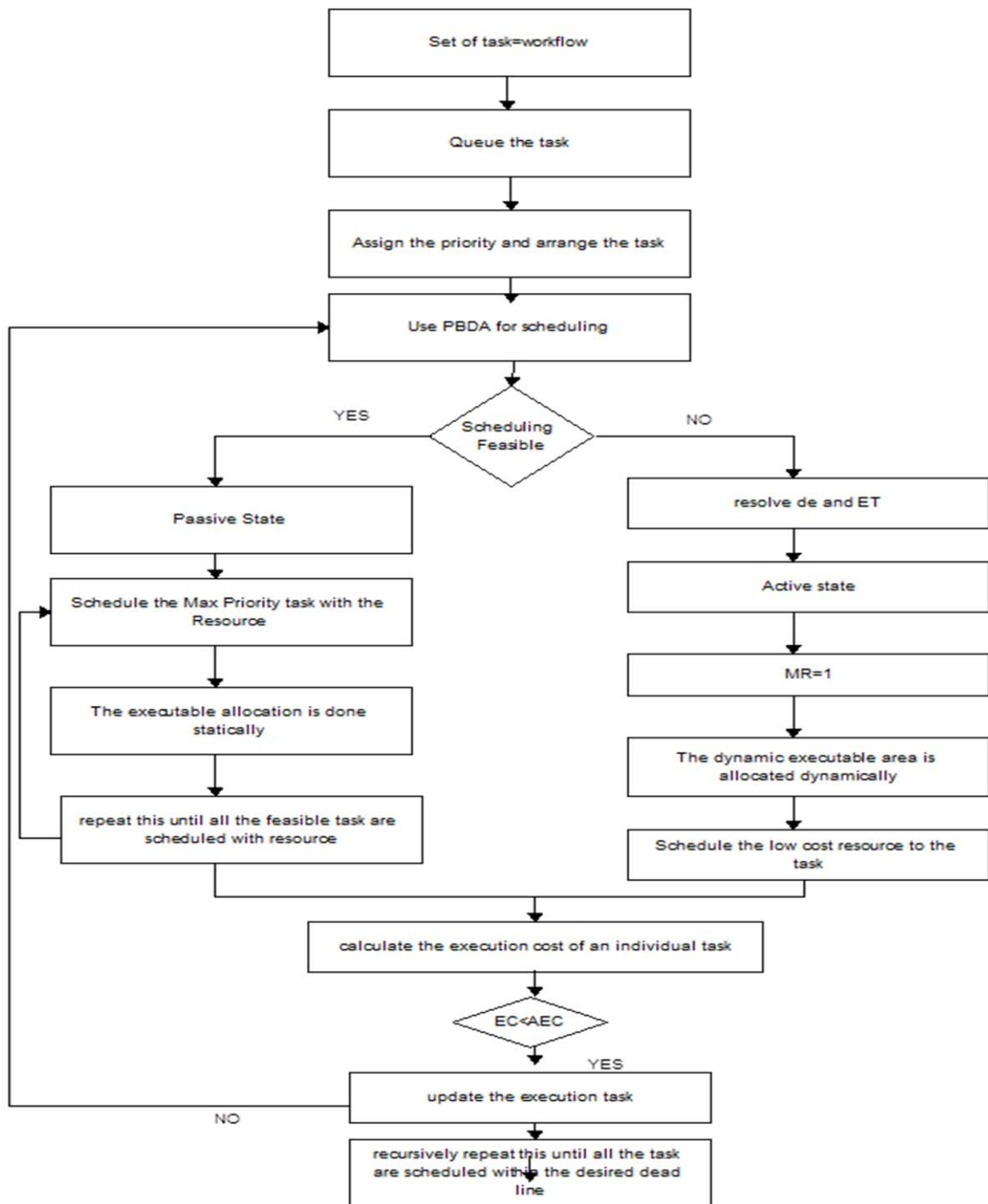
Fig. 1 Algorithm description for PBD
