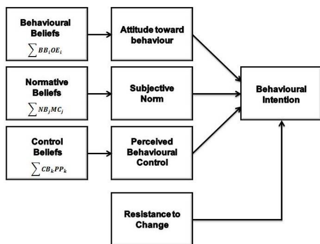
Fig. 1 Theory of Planned Behaviour (TPB) model with Resistance to Change variable
