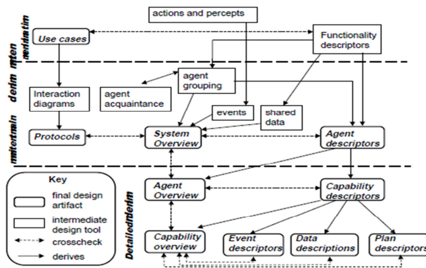
Fig. 1 Prometheus methodology phases [9]
