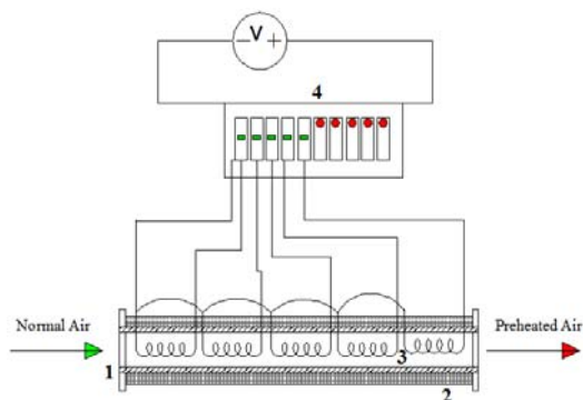
Fig. 2 Air preheating unit (1-Steel pipe, 2-Insulation, 3-Electrical heaters, 4-Automatic electric switches)
