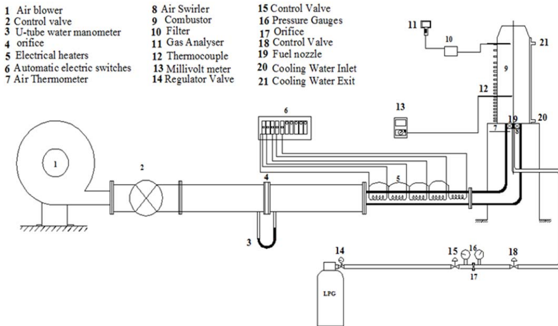
Fig. 1 Experimental test rig
