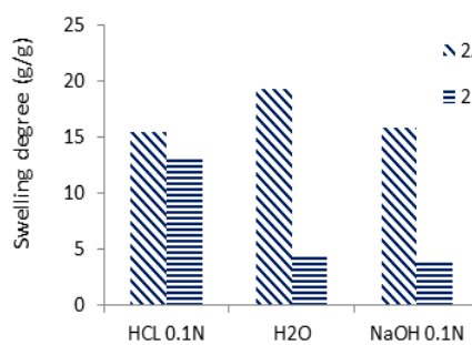
Fig. 3 Swelling degree of non-cross-linked (2A) and cross-linked glucomannan-carrageenan (2B) at various media
