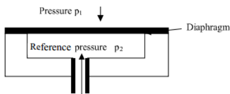
Fig. 3 Differential pressure sensor [11]
