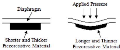
Fig. 6 Deformation of piezoresistive material
