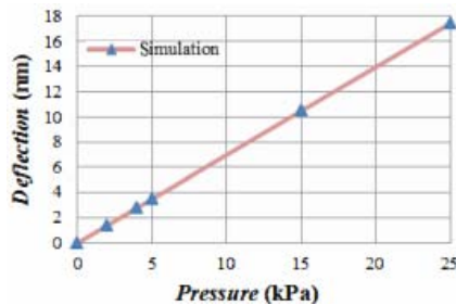
Fig. 20 Linear relation between diaphragm deflection and pressure [21]
