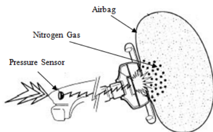
Fig. 14 MEMS pressure sensor in airbag firing system
