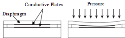
Fig. 10 Structure of capacitive sensor
