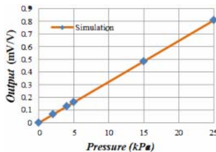
Fig. 21 Linear relation between sensor output and pressure [21]
