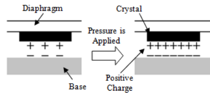
Fig. 8 Piezoelectric pressure sensor
