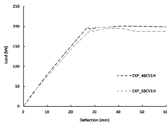
Fig. 9 Load-deflection curves of test specimens heated for 1 hour
