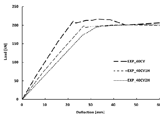
Fig. 11 Load-deflection curves according to heating time difference
