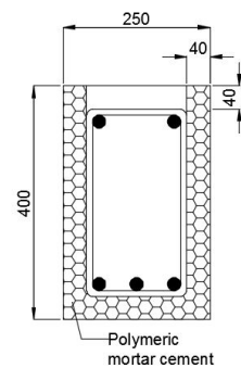
Fig. 4 Section of rehabilitated specimen (unit: mm)
