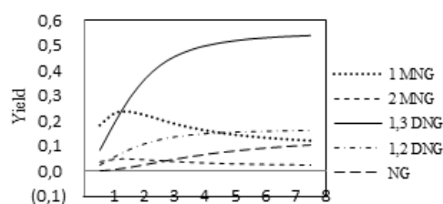
Fig. 3 Effect of mol ratio of nitric acid/glycerol to conversion of Products ( \text{HNO}_3 71.35%, 20° C)
