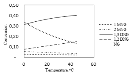
Fig. 5 The conversion of products of nitration at various temperature (concentration of HNO 3 71.35%, mol ratio of 2/1)
