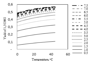
Fig. 6 The conversion of 1, 3- DNG at various temperatures (at various mol ratios) and nitric acid concentration of 71.35%
