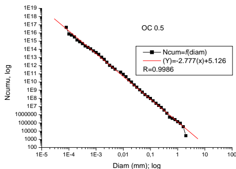
Fig. 2 Fractal line of OC 0,5, FD=2,777
