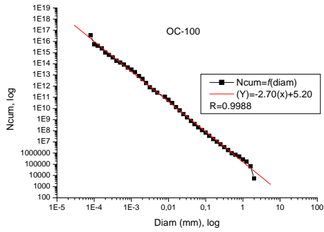
Fig. 7 Fractal line of OC-100, FD=2,70
