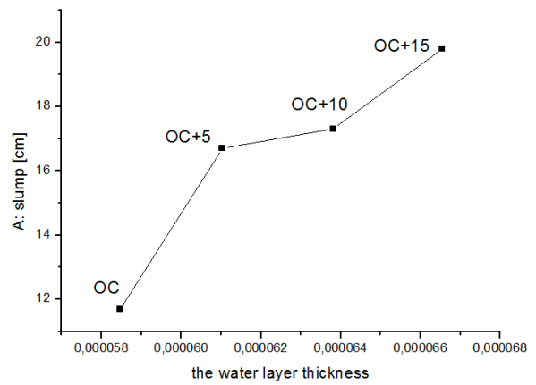
Fig. 15 Sub-program 3: OC+ water, A=f(T WL )
