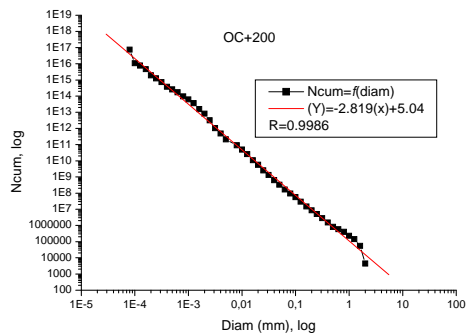
Fig. 9 Fractal line of OC+200, FD=2,819
