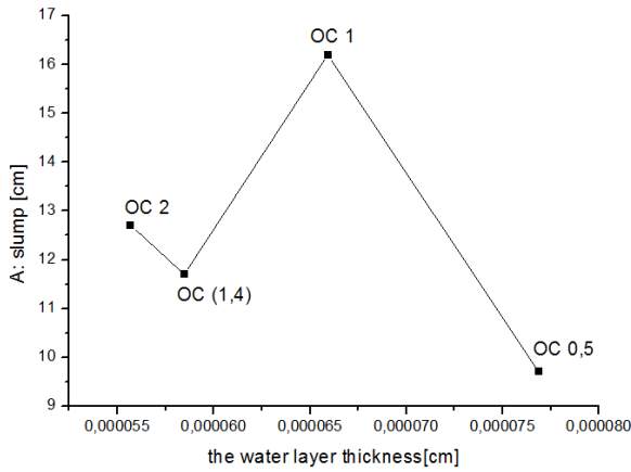
Fig. 13 Sub-program 1: OC+G/S, A=f(T WL )
