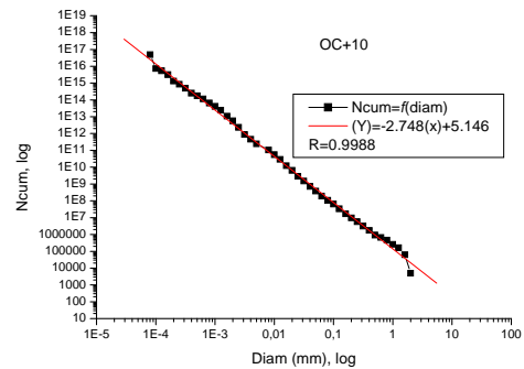
Fig. 11 Fractal line of OC+10, FD=2,748
