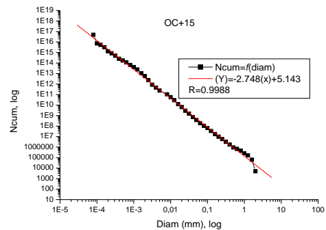
Fig. 12 Fractal line of OC+15, FD=2,748
