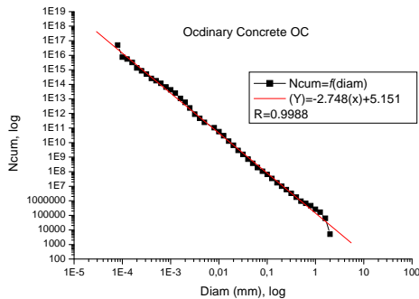
Fig. 1 Fractal line of control concrete OC, FD=2,748
