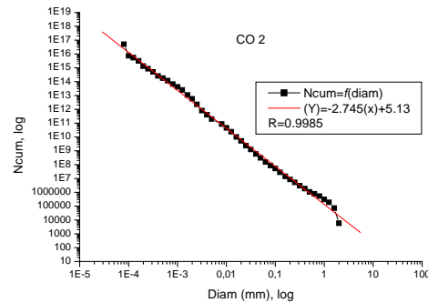
Fig. 4 Fractal line of OC 2, FD=2,754
