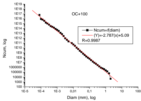
Fig. 8 Fractal line of OC+100, FD=2,787
