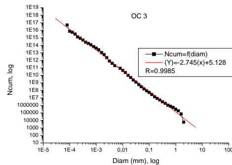
Fig. 5 Fractal line of OC 3, FD=2,754
