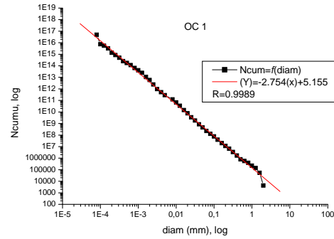
Fig. 3 Fractal line of OC 1, FD=2,754
