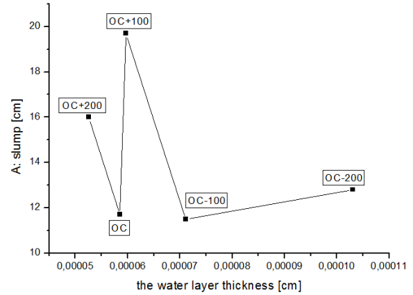
Fig. 14 Sub-program 2: OC+ cement, A=f(T WL )
