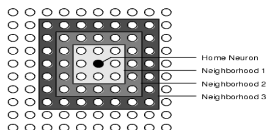
Fig. 3 Rectangular neighborhood in home neuron
