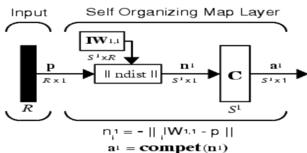
Fig. 1 Block diagram of SOFM network
