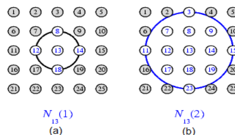
Fig. 2 Circular neighborhood in neuron 13
