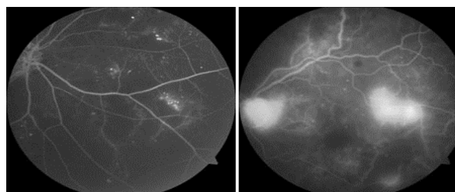
Fig. 17 Failed Images
