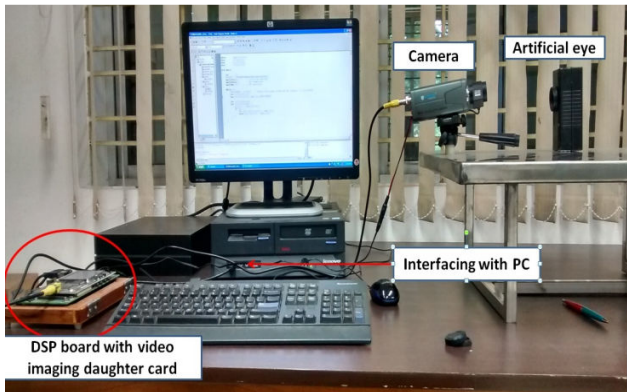
Fig. 7 Experimental setup
