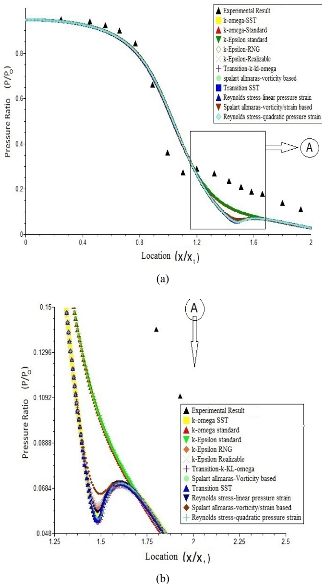
Fig. 3 Comparison of experimental and computational results of flow through a CD nozzle (NPR = 8.945) using various models showing the Centerline pressure: (a) Comparison of experimental and computational results of axial pressure ratio of a CD nozzle using various models (b) Enlarged view of centerline pressure corresponding to Fig. 3 (a)
