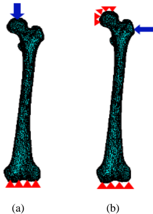
Fig. 2 Application of loading and boundary conditions during (a) the single-leg stance, and (b) the sideways fall
